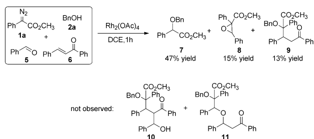
Scheme 3. Intermolecular four-component competitive reaction.
